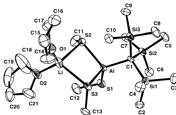
Fig. 1 Molecular structure of [Li(thf) 2 {Al[C(SiMe 3 ) 3 ](SMEx) 3 } 2 .
